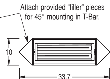
Face View (45° Mounting)
